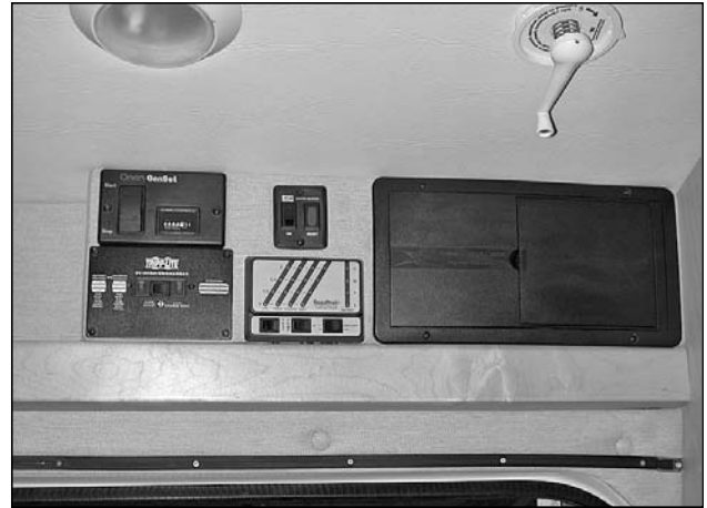
Picture E-P1: Monitor panel, water heater switch, 110V/12V distribution panel and optional generator control switch.
