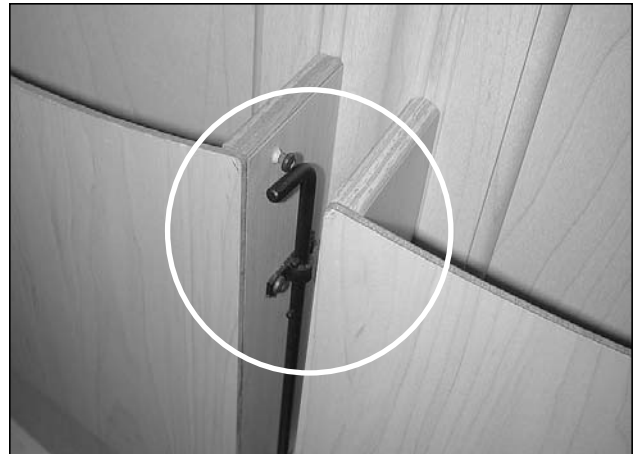
Picture B-P21: Front bathroom door, (in transit) locking pin in the locked position.
